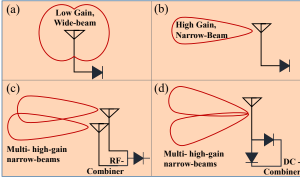
Fig. 5. Rectenna topologies based on the antennas' radiation patterns. (a): Omni-directional antenna. (b): High-gain directional. (c): Multi-high-gain narrow-beam antenna with RF combining. (d): Multi-high-gain narrow-beam with DC combining.
