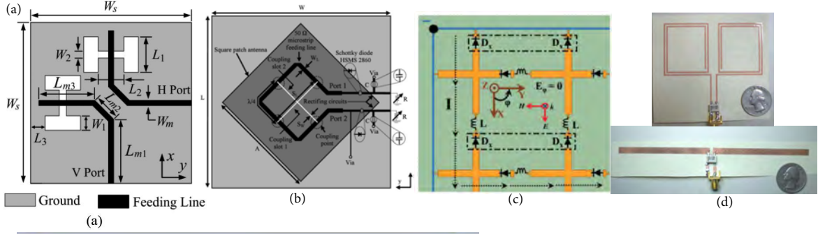
Fig. 7. Polarization independent rectennas: A: dual-LP slot [47], b: dual-CP slot [37], c: dual-LP cross-dipole array [58], d: dual antennas for harvesting near field H- (top) and E- (bottom) fields [105].
